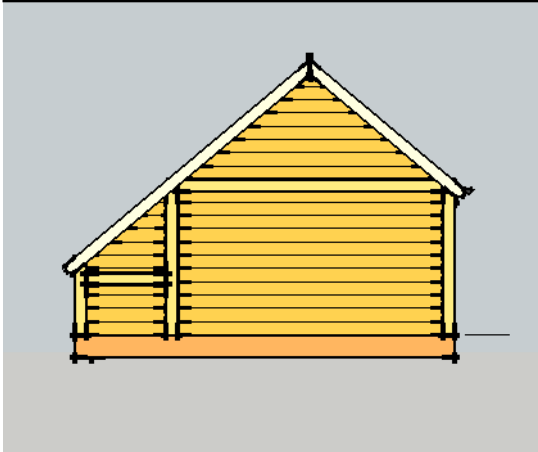
Rear Elevation 1:100
