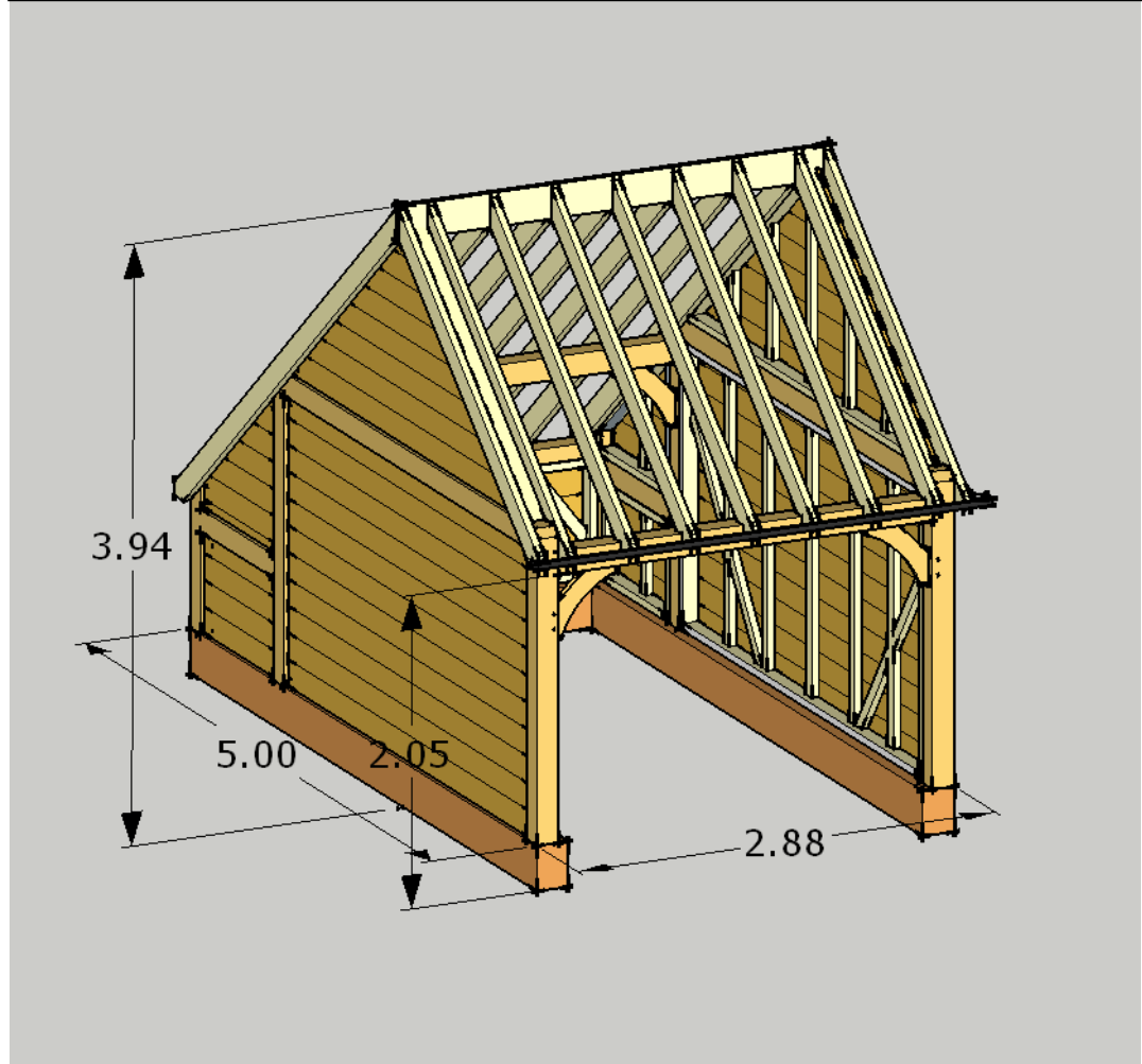
Isometric 1:50
