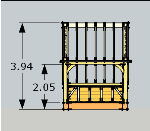
Side Elevation 1:100
